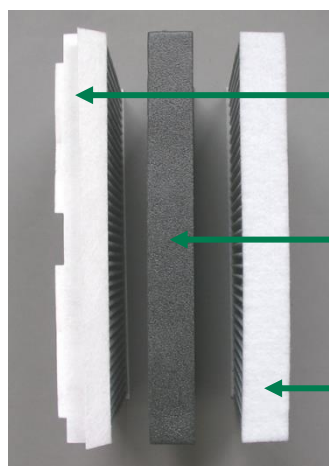
New MANN-FILTER design with modified material of frame
